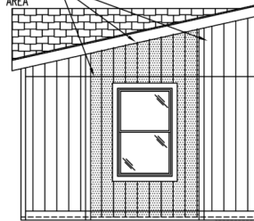
OPTIONAL UPGRADED HITCH END ELEVATION
